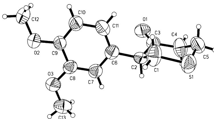
Figure 3. ORTEP representation of the structure of compound 1b in the solid state.
