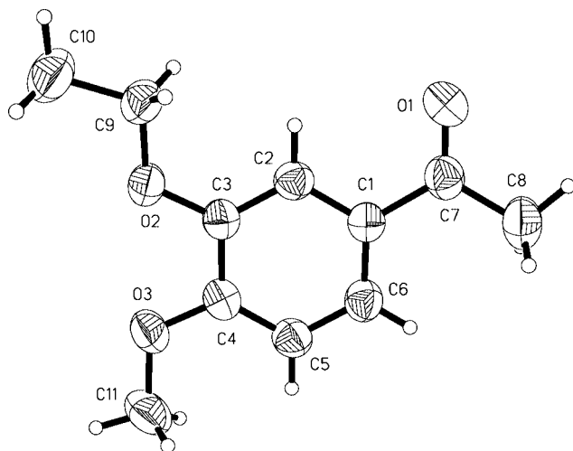
Figure 1. ORTEP representation of the structure of compound 7b in the solid state.
