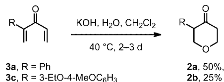
Scheme 6. Synthesis of 3-aryl-substituted tetrahydropyran-4-ones 2 by double conjugate addition.
