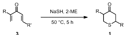
Scheme 5. Synthesis of 3-aryl-substituted tetrahydrothiopyran-4-ones 1 by double-conjugate addition. For yields and substituents see Table 3.
