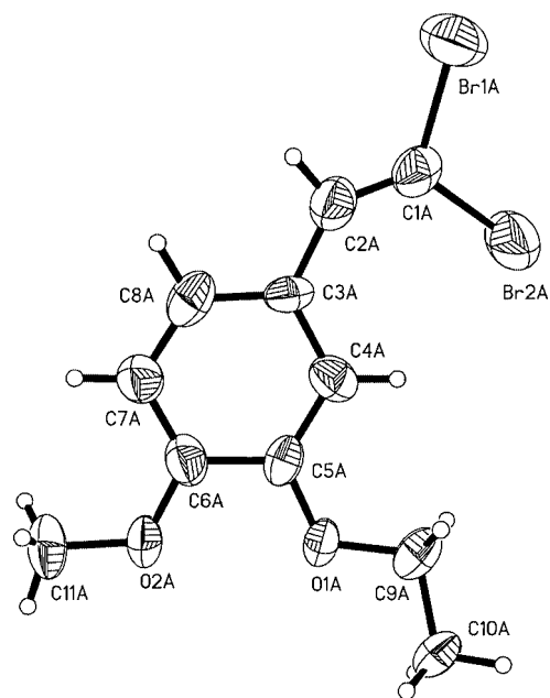
Figure 2. ORTEP representation of the structure of compound 11b in the solid state.
