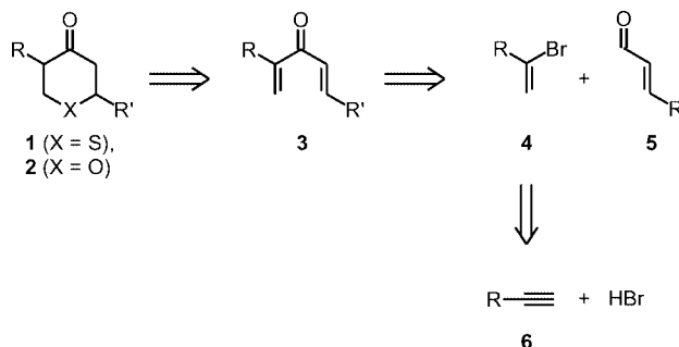
Scheme 1. Strategy for the preparation of 3-aryl-substituted tetrahydrothiopyran-4-ones 1 and tetrahydropyran-4-ones 2 by double-conjugate addition. Retrosynthesis of the divinyl ketones 3 by \alpha -bromostyrene derivatives 4 to alkynes 6 . R = electron-rich aryl, R' = H, Ph.
