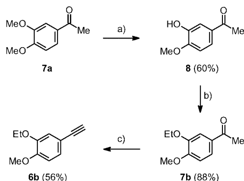
Scheme 2. From veratropheneone ( 7a ) to alkyne 6b by dealkylation, alkylation, and elimination. Reagents and conditions: a) H_2SO_4 (concd.), 65 °C, 46 h; 60% ( 8 ). b) EtBr, K_2CO_3 , DMF, 100 °C, 6 h; 88% ( 7b ). c) 1. LDA, THF, –78 °C, 1 h; 2. (EtO)_2P(O)Cl , 23 °C, 3 h; 3. LDA, –78 °C, 23 °C, 3 h; 56% ( 6b ).
