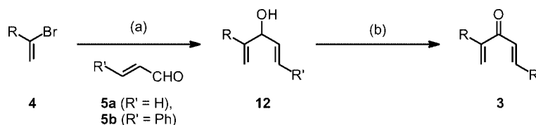
Scheme 4. Synthesis of divinyl ketones 3 from \alpha -bromostyrenes 4 . Reagents and conditions: (a) 1. n BuLi, THF, 1.5 h, -78^\circ\text{C} ; 2. aldehyde 5 , 1.5 h, -78^\circ\text{C} ; (b) excess \text{MnO}_2 , \text{CH}_2\text{Cl}_2 , 60 min, 23^\circ\text{C} .
